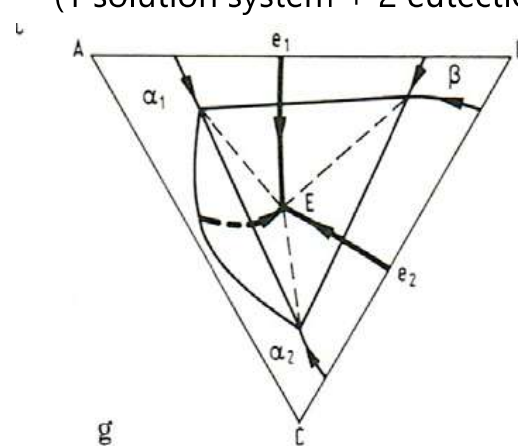
ternary eutectic (1 solution system + 2 eutectics)
