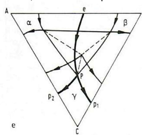
ternary peritectic (1 eutectic + 2 peritectics)
