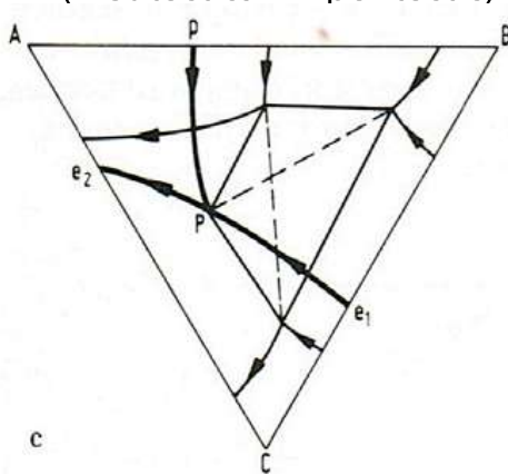
ternary quasi-peritectic (2 eutectics + 1 peritectic)
