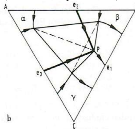
ternary quasi-peritectic (from 3 binary eutectics)
