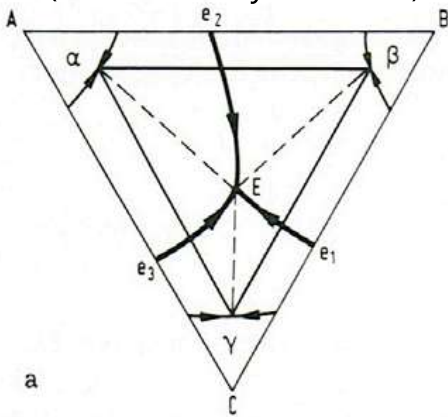
ternary eutectic (from 3 binary eutectics)
