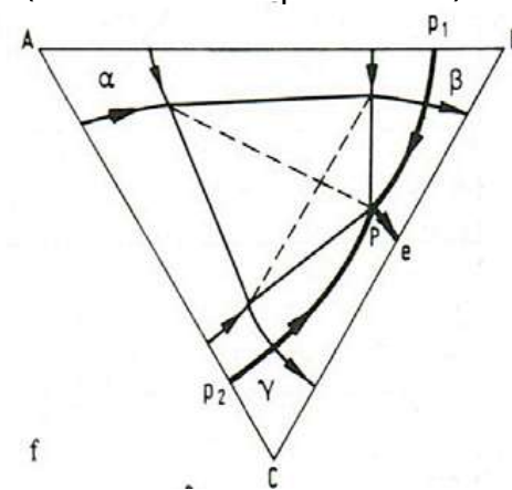
ternary quasi-peritectic (1 eutectic + 2 peritectics)
