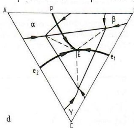
ternary eutectic (2 eutectics + 1 peritectic)
